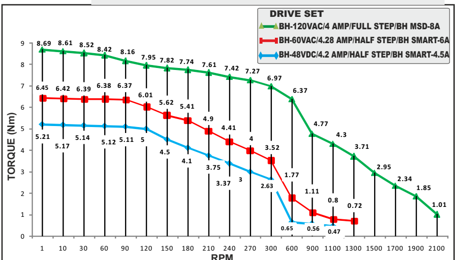
STEPPER MOTOR - BH86SH 150- 4004 AKS-FLP
