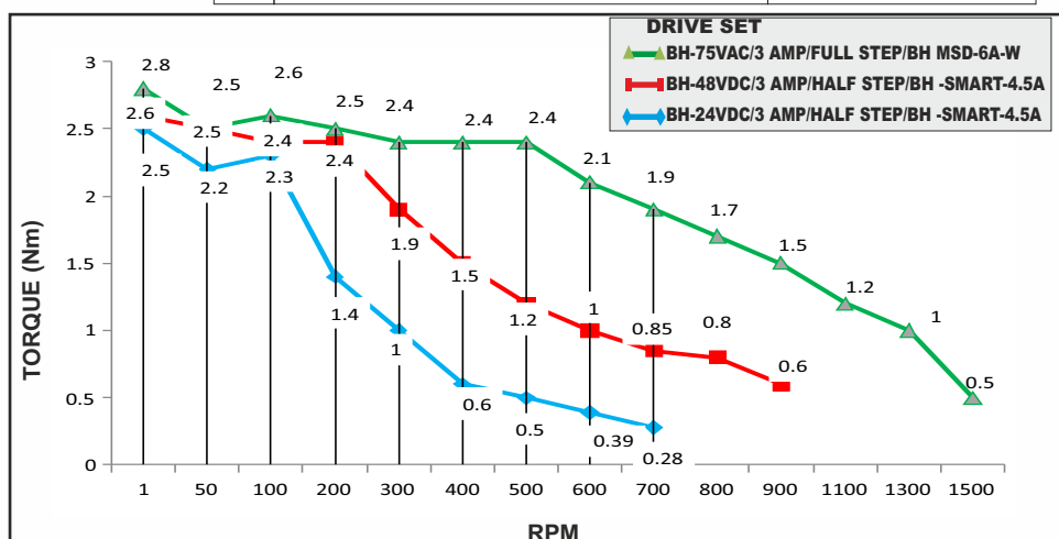
STEPPER MOTOR - BH86SH65-3004AK
