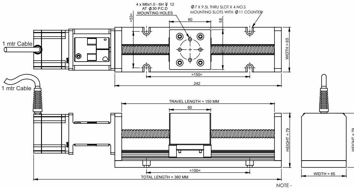
Regular slide without bellow cover
