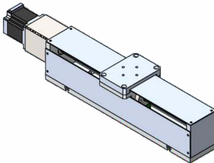
X SLIDE WITH SHEET METAL COVER
