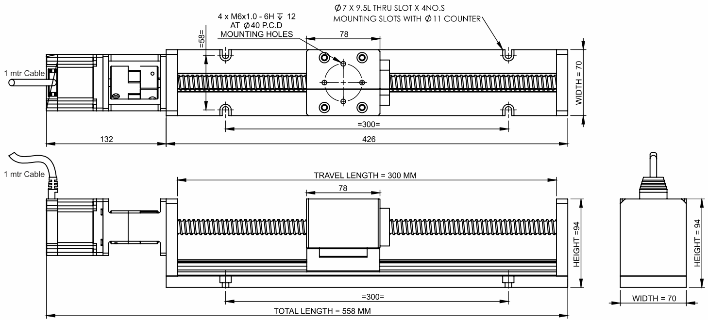
Regular slide without bellow cover
